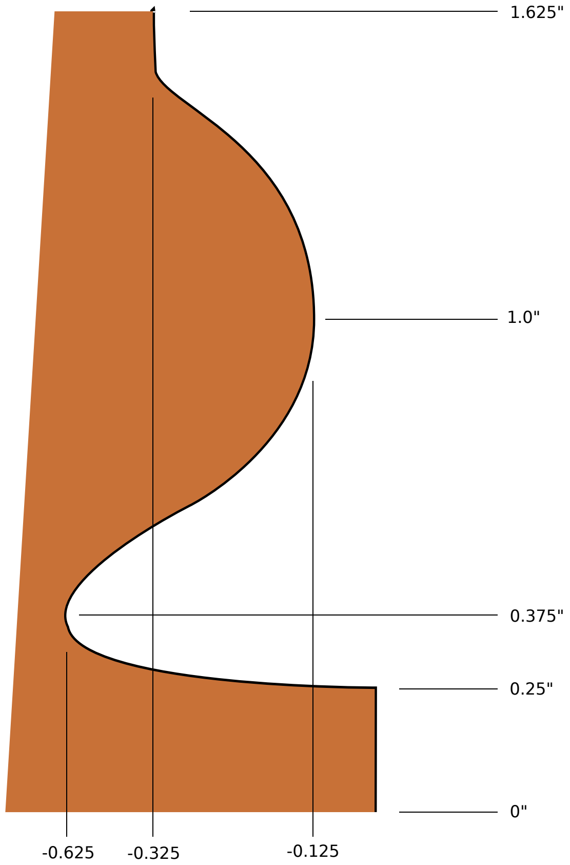
Ben Dugan Porchg Column Base Profile
